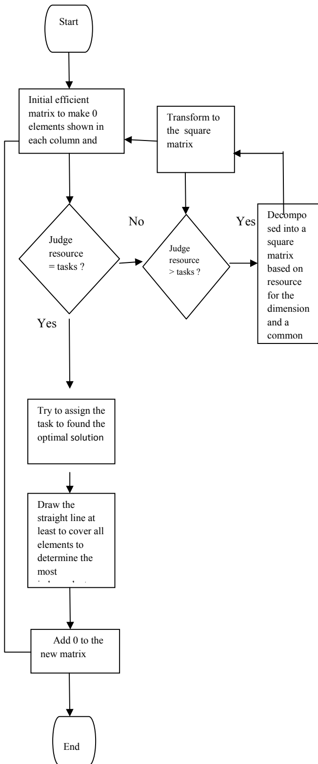
Fig 2. Steps in Hungarian Algorithm
