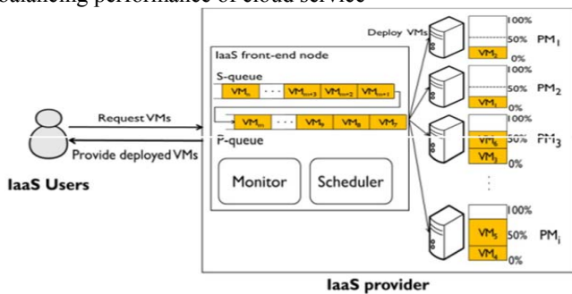
Fig 1. Architecture of IaaS Front End Node
