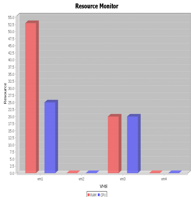
Fig 3. Resource Monitoring
